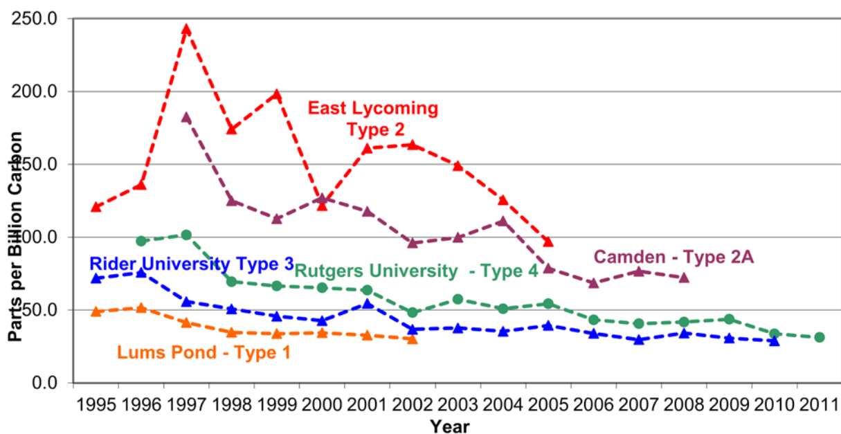
Figure 3 Philadelphia Region Total Non-methane Organic Carbon (TNMOC) Seasonal Average 1995-2011
